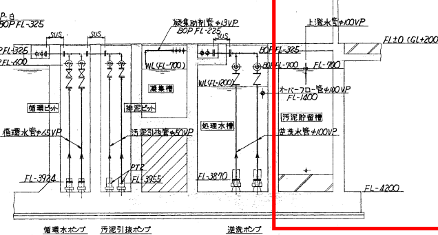
“C-C”断面図
